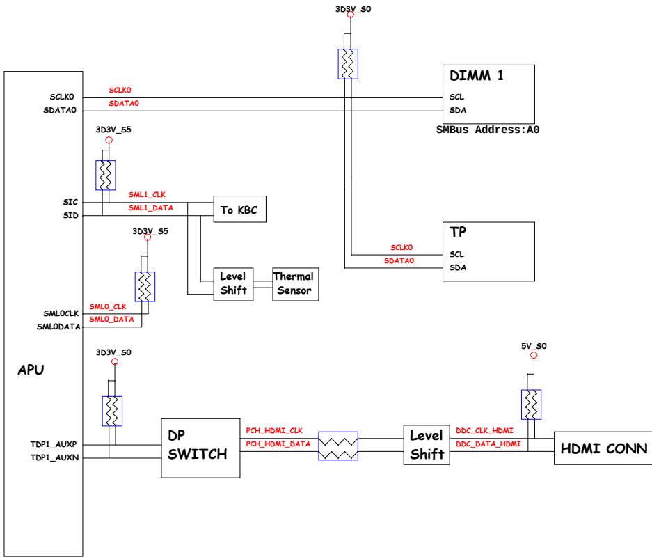
APU SMBus Block Diagram
